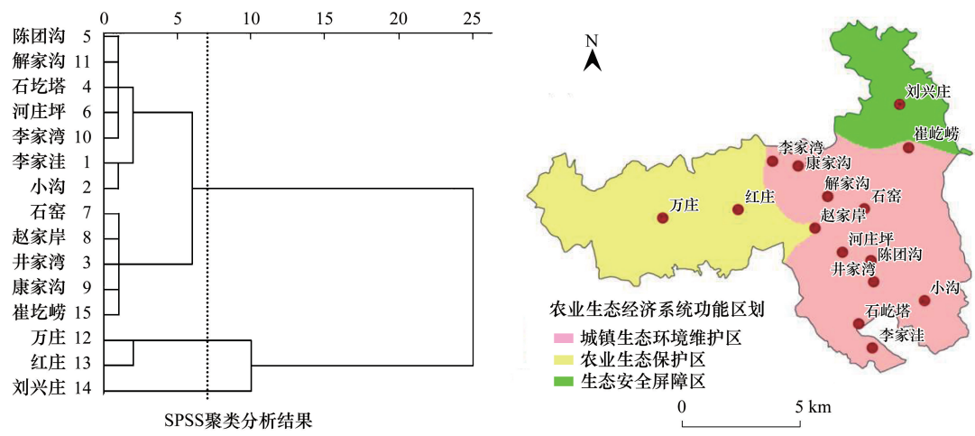
图 6 研究区农业生态经济系统功能分区 Fig.6 Functional division of agro-ecological economic system in the study area
