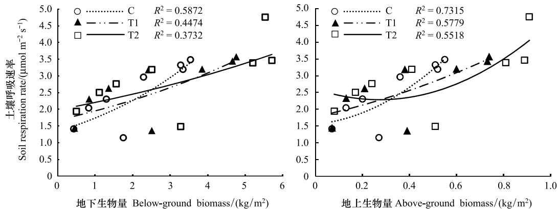
图7 土壤呼吸速率与生物量间的曲线拟合 Fig.7 Curve fitting between soil respiration rate and biomass
