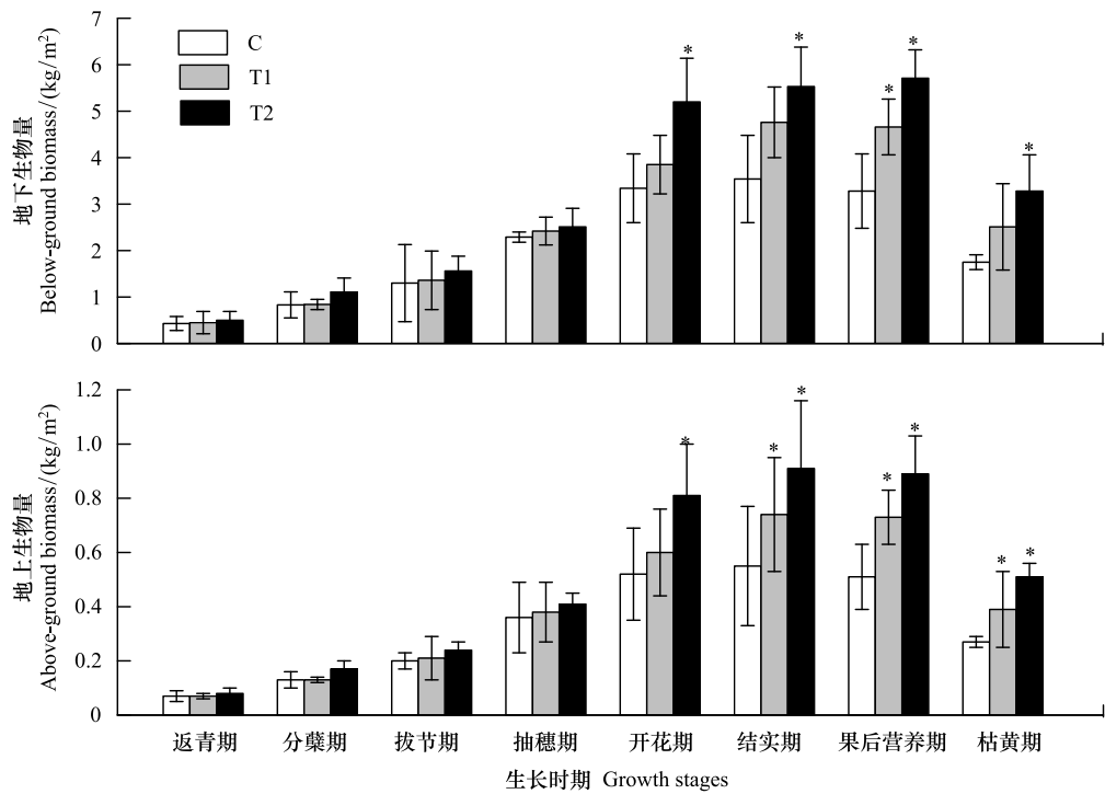
图 6 不同处理下地下根系生物量和地上生物量的变化 (平均值±标准差) Fig.6 Effects of experimental warming on below-ground biomass and above-ground biomass (mean±SE)
