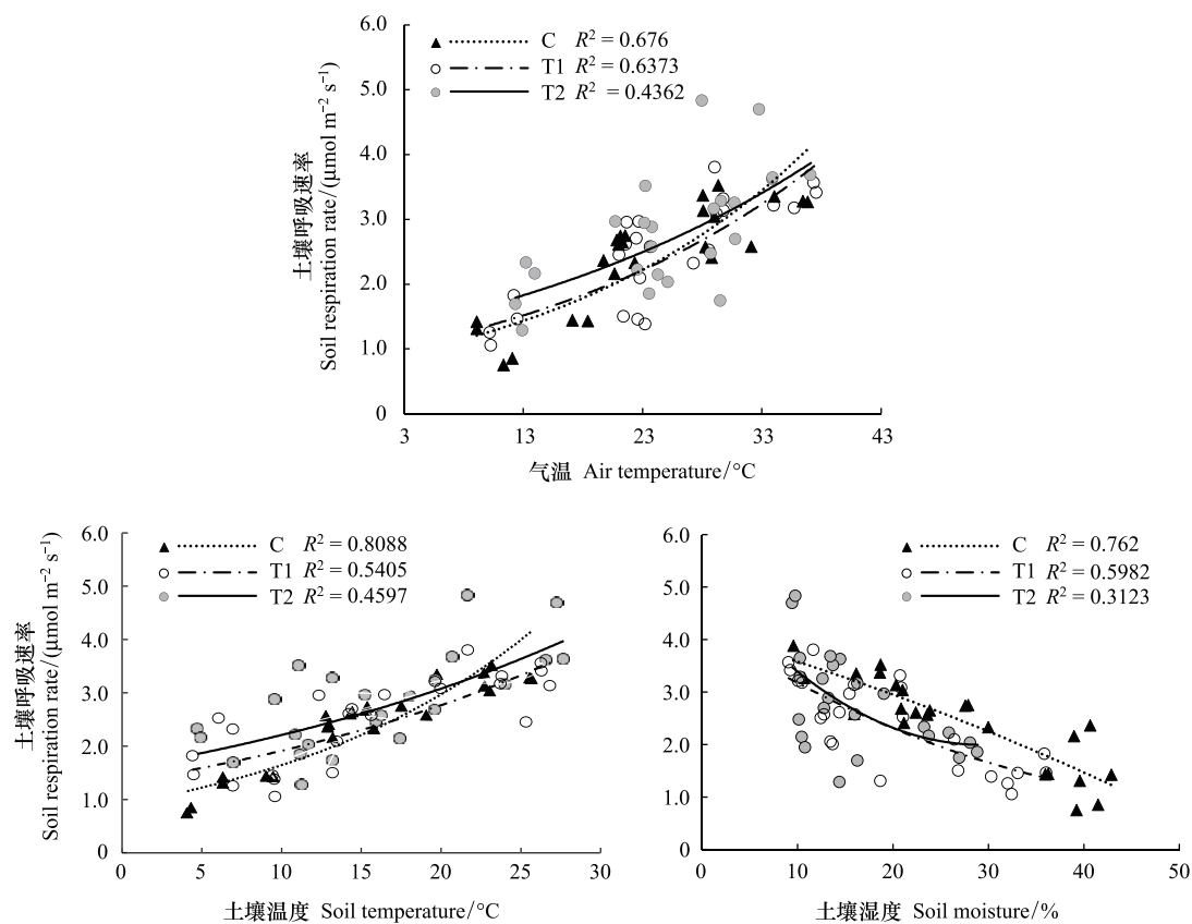
图 5 土壤呼吸速率与环境因子间的曲线拟合 Fig.5 Curve fitting between soil respiration rate and different environmental factors
