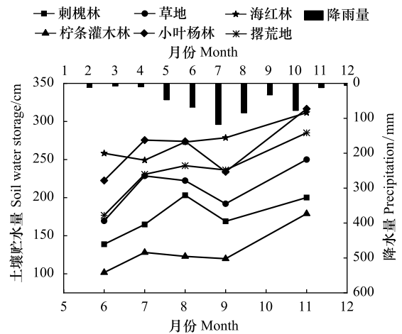
图 3 监测期不同土地利用方式土壤贮水量与降水量变化 Fig.3 The variation of soil water storage in different land-use types and precipitation
