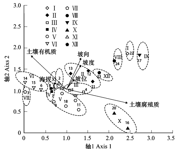
图 5 东拉山短丝木犀植物群落 24 个样地的 DCCA 二维排序图 Fig.5 DCCA two-dimensional sorting map of 24 plots of plant community of the Osmanthus serrulatus
