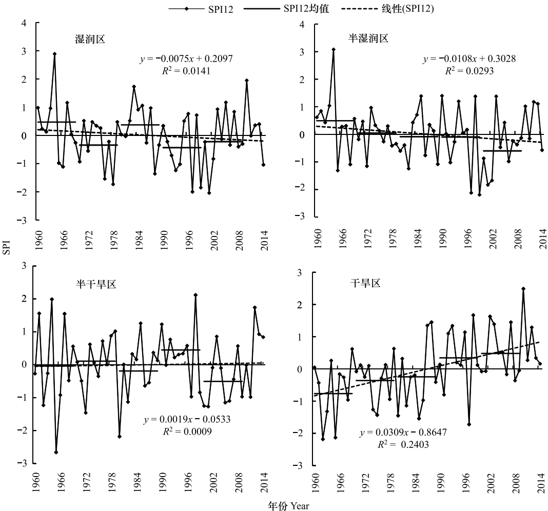
图 5 1960—2014 年不同干湿区年 SPI 变化 Fig.5 Evolution of annual SPI in different dry and wet areas from 1960 to 2014
