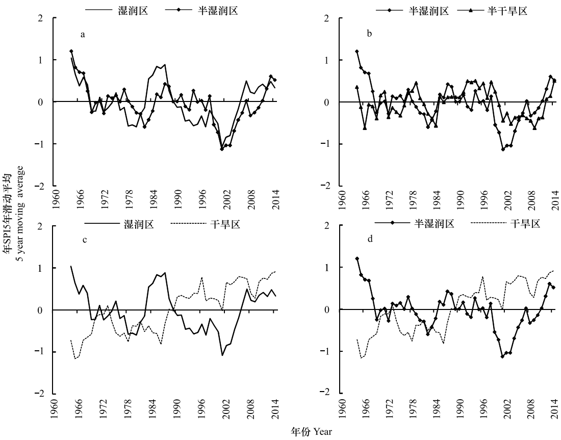
图 6 不同干湿区年 SPI5 年滑动平均波动过程图 Fig.6 Evolution of annual SPI 5year moving average in different dry and wet areas
