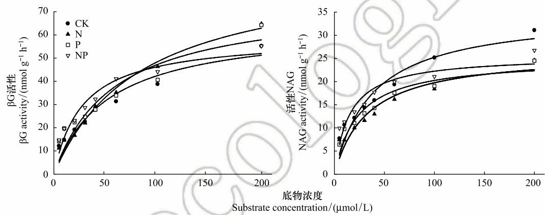
图 2 氮磷添加条件下 β-1,4-葡萄糖苷酶 (βG) 和 β-1,4-N-乙酰葡萄糖氨糖苷酶 (NAG) 米氏方程拟合结果 Fig.2 Michaelis-Menten equation of β-glucosidase (βG) and N-acetyl-glucosaminidase (NAG) under N and P additions
