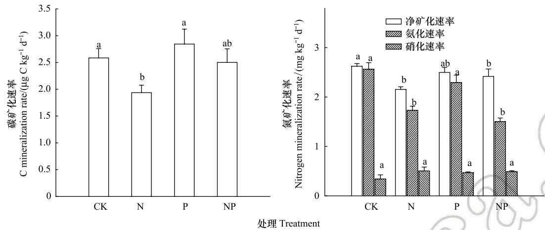
图 1 氮磷添加对土壤碳氮矿化速率的影响 Fig.1 The effects of nitrogen and phosphorus additions on the rates of soil carbon and nitrogen mineralization
