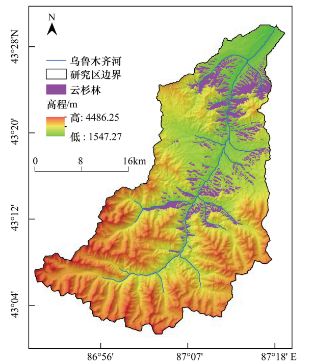
图2 云杉林空间分布图 Fig.2 The spatial distribution map of spruce forest
