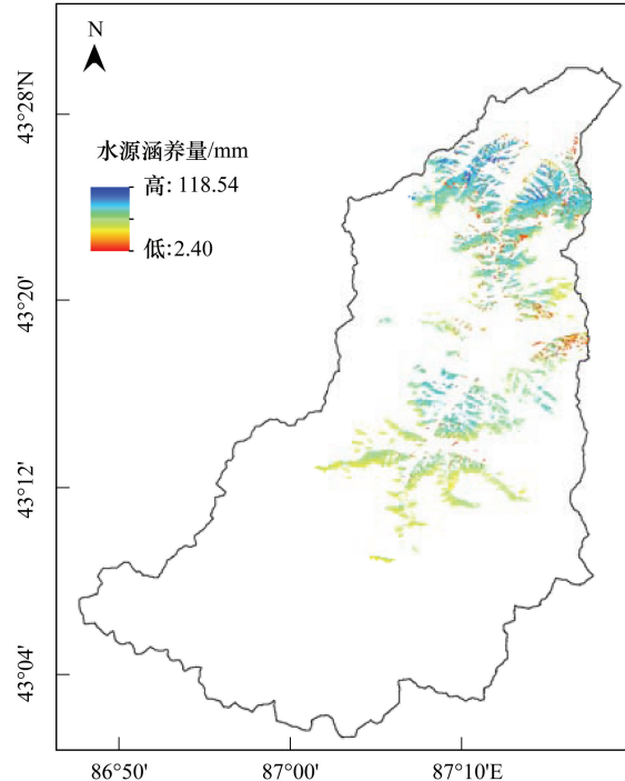
图 5 云杉林区水源涵养分布图 Fig.5 Water conservation in forest region
