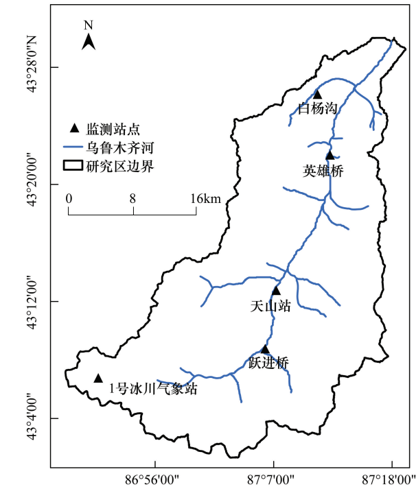
图1 研究区示意图 Fig.1 The location of the study area
