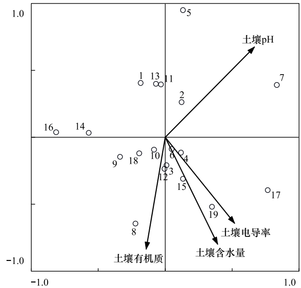
图 3 恒湖农场茶叶港草洲 19 个样地 RDA 排序图 Fig.3 RDA ordination of 19 sample plots in Chayegang marshland near Henghu farm
