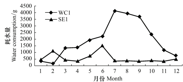
图 4 在地表覆盖物下意杨蒸腾耗水量和土壤蒸发量月际变化曲线 Fig.4 Monthly change curves of water consumption of poplar and soil evaporation under land covering Soil evaporation 1 (SE 1 ) 为栽植意杨的土壤蒸发量, Water consumption 1 (WC 1 ) 为有地表覆盖物下的意杨蒸腾耗水量
