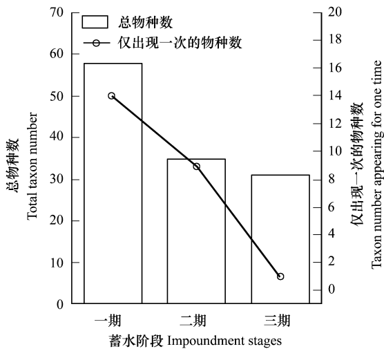
图 4 不同蓄水阶段香溪水库湾底栖动物总物种数及出现一次的物种数对比 Fig.4 Total taxon number in the Xiangxi Bay and the number of taxon appearing for one time during different impoundment stages
