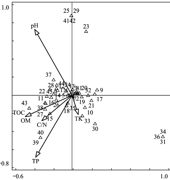
图 2 中小型土壤动物与土壤环境典范对应分析排序图 Fig. 2 Canonical correspondence analysis ordination of meso-micro soil fauna and soil environment
