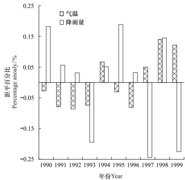
图 11 1990s 研究区气候因子偏差分析 Fig.11 Deviation analysis of climatic factors in 1990s
