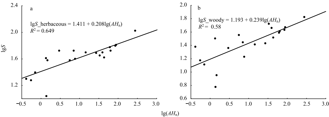
图 3 草本和木本植物的种—面积—生境类型关系模型拟合 Fig.3 The species-area-habitat relationship (SAH n R) of the herbaceous (a) and woody plants (b) using
