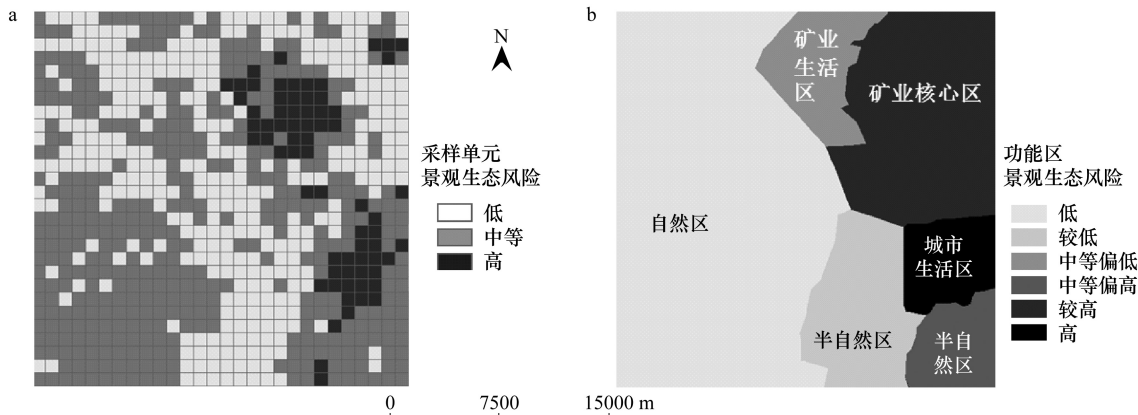
图2 矿区采样单元与功能分区景观生态风险空间分布 Fig.2 landscape eco-risk of sample units and the different functional zones of opencast mining area
