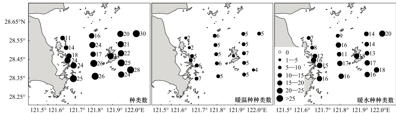
图 3 7 月浮游动物种类数分布 Fig. 3 Distribution of species richness for zooplankton in July, 2010
