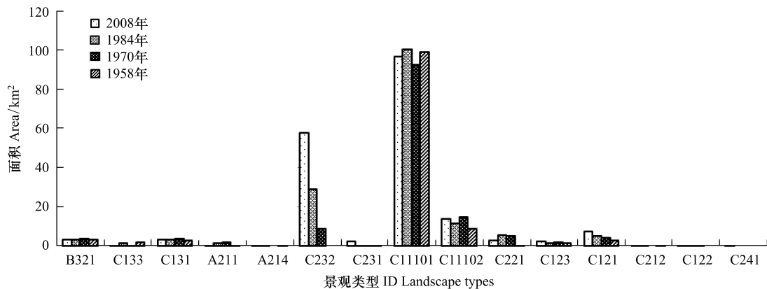
图5 大洋河河口不同年人为干扰度景观类型面积 Fig. 5 Ara of human disturbed landscape types in different years in Dayang estuary
