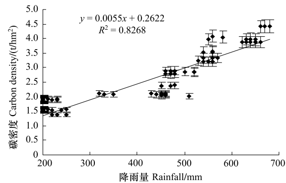
图 7 年草地碳密度与降雨量变化 Fig.7 Changes between carbon density and rainfall of enclosed 11a grassland
