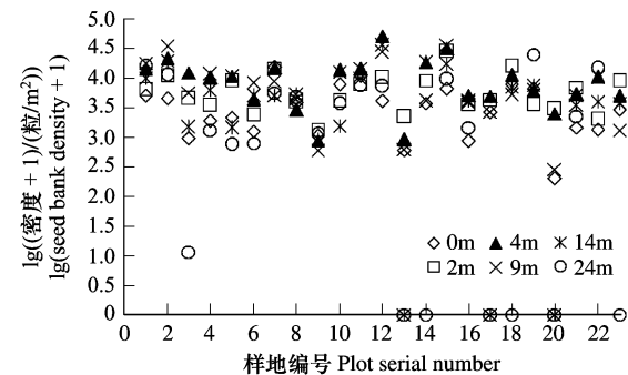
图 4 不同样地距公路不同距离的紫茎泽兰土壤种子分布 Fig. 4 The patterns of soil seed density of E. adenophorum at different distance to roads at different plots
