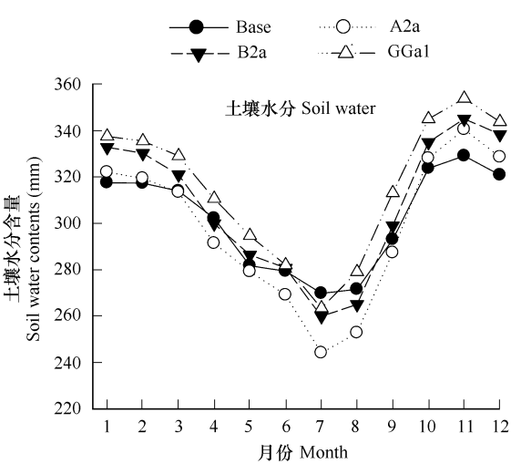
图5 土壤水分的月变化 Fig. 5 The change of monthly soil water contents
