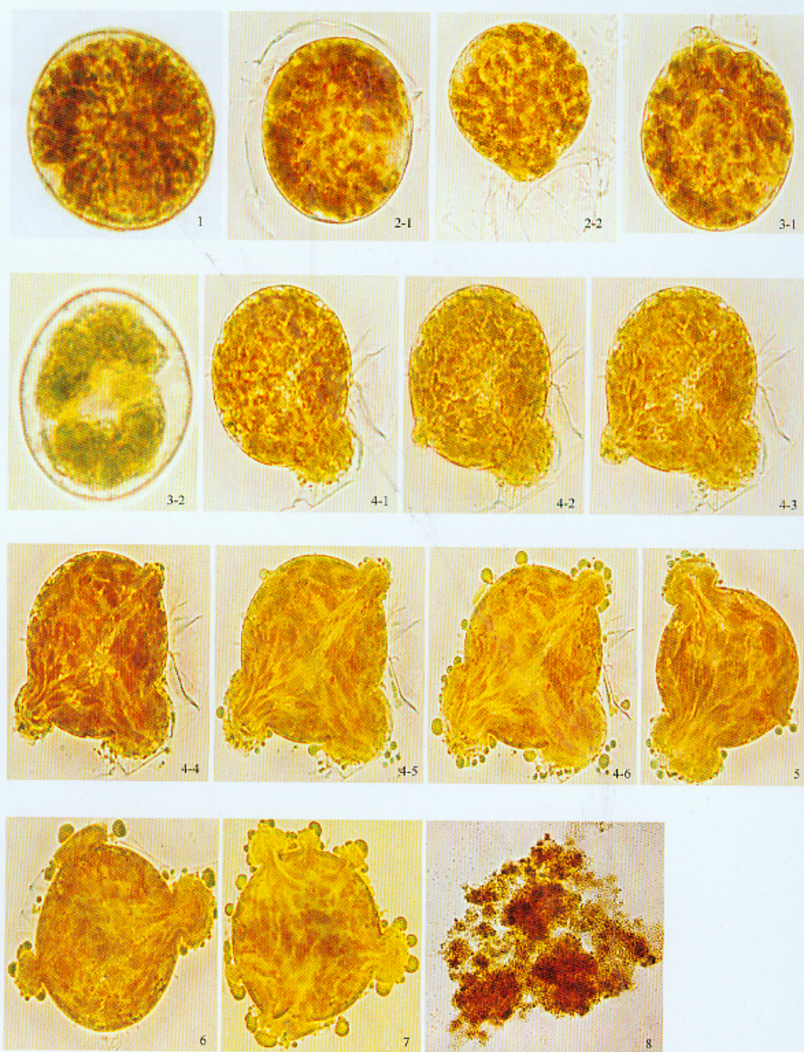
图1 塔玛亚历山大藻培养液中加入 2216E 后藻细胞形态变化 Fig. 1 Variation of algae cell structure after the 2216E medium was added to A. tamarensis culture
